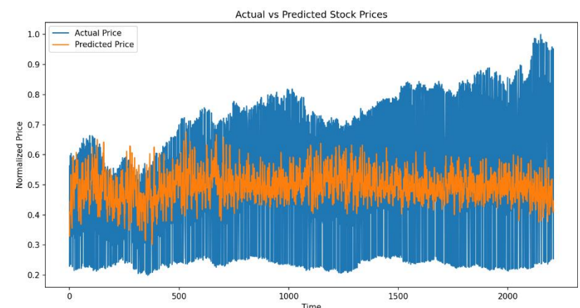
Fig 8.1. Graph Plotting the variation in Actual Stock Prices and Predicted Stock Prices
